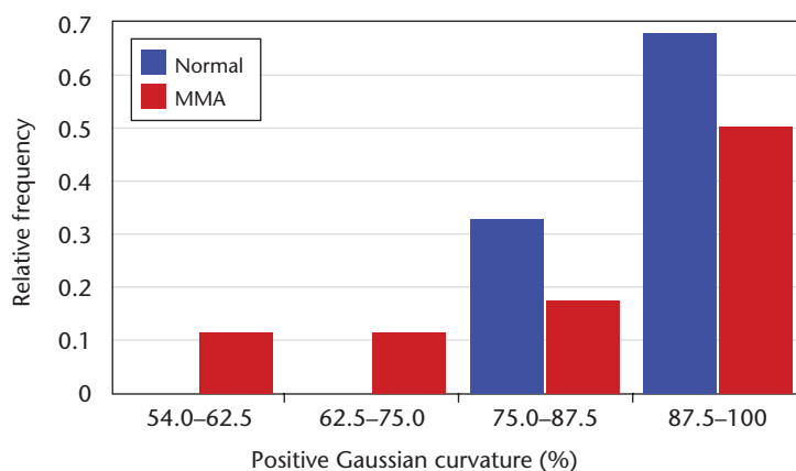
Figure 6. Plotting the percentage of positive Gaussian curvature yields a size-invariant metric that implies two distinct populations. This suggests that mitochondrial shape is possibly an early indicator of MMA.
